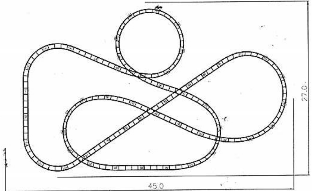
Topview Scale 1:250
